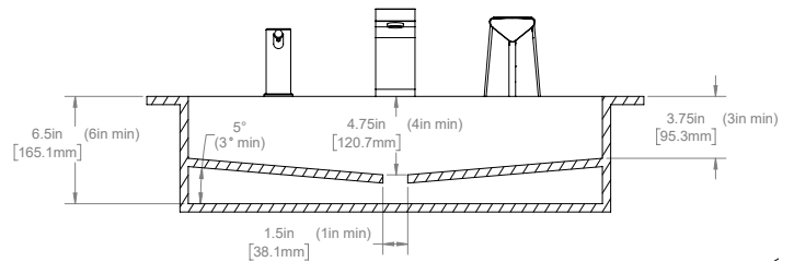
OPTIMAL SINK DIMENSIONS (horizontal slope)
