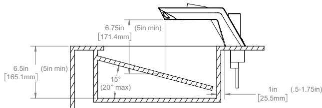
OPTIMAL SINK DIMENSIONS (forward slope)
