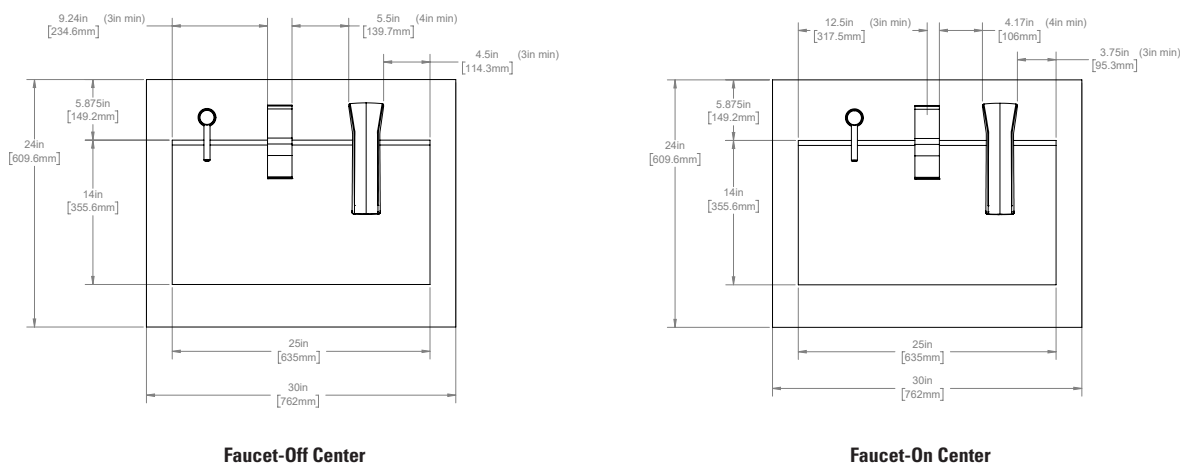
Faucet-Off Center
