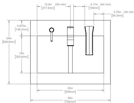
Faucet-On Center
